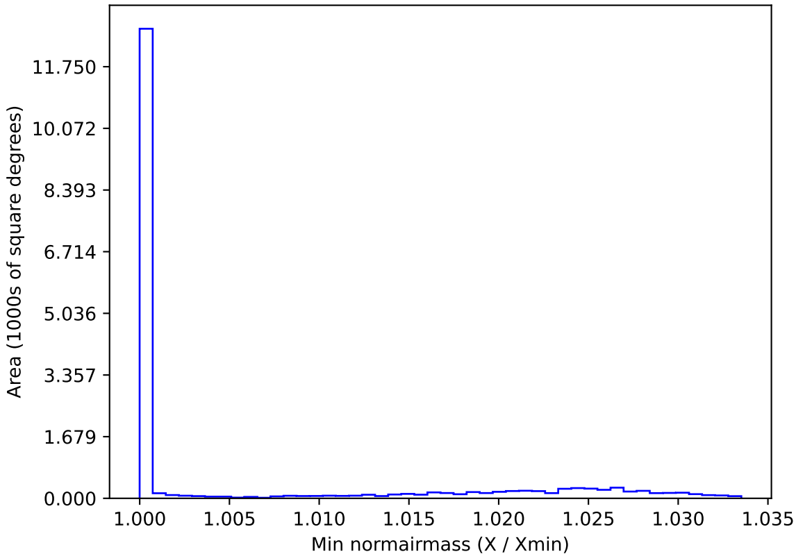
roll_pause_mjdp60_v3.4_10yrs WFD i band: Min normairmass
