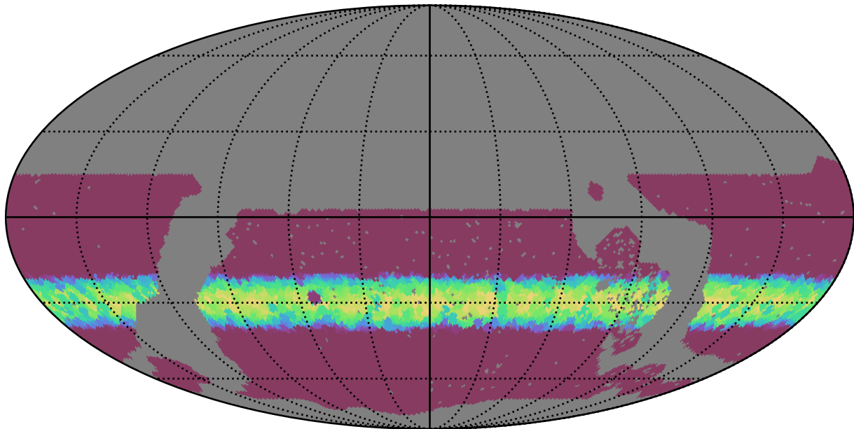
roll_pause_mjdp60_v3.4_10yrs WFD all bands: Min normairmass
