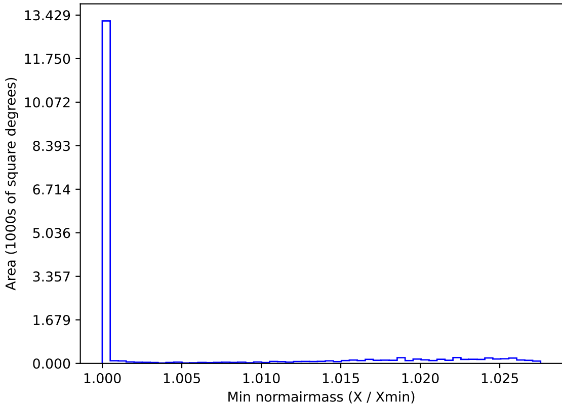
roll_pause_mjdp60_v3.4_10yrs WFD all bands: Min normairmass
