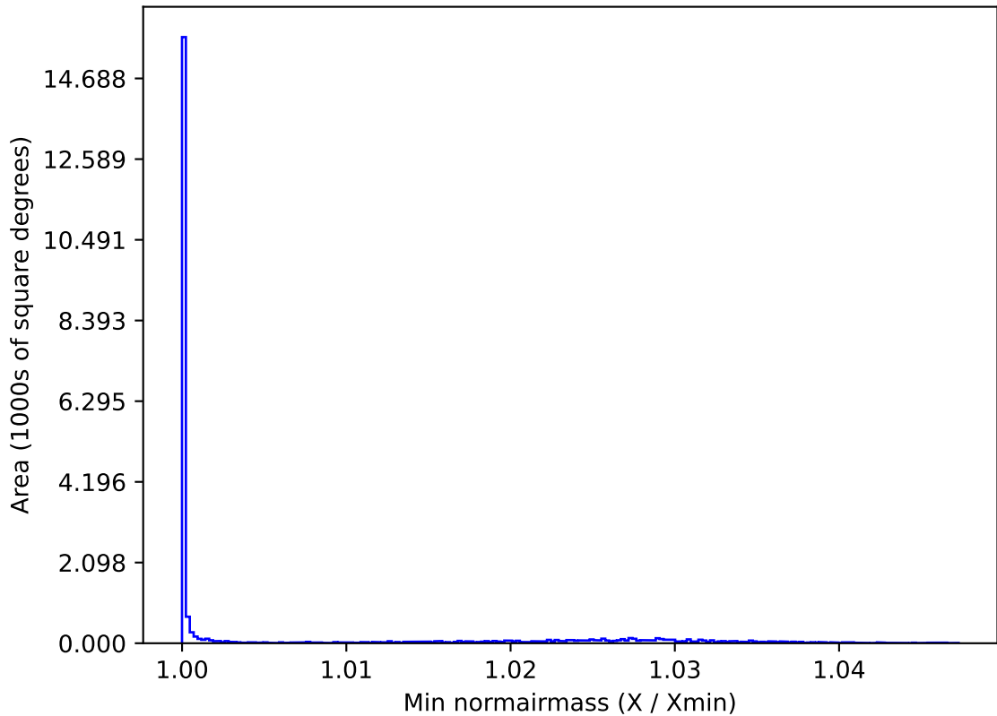
roll_pause_mjdp60_v3.4_10yrs All sky y band: Min normairmass
