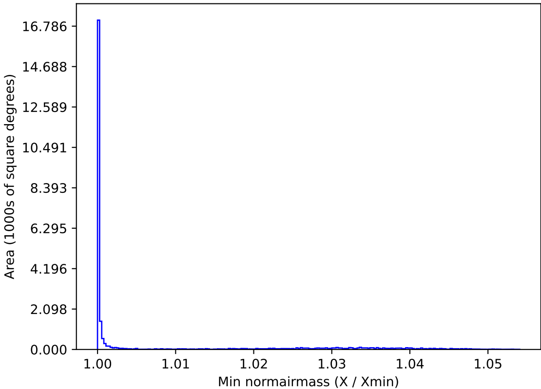
roll_pause_mjdp60_v3.4_10yrs All sky g band: Min normairmass
