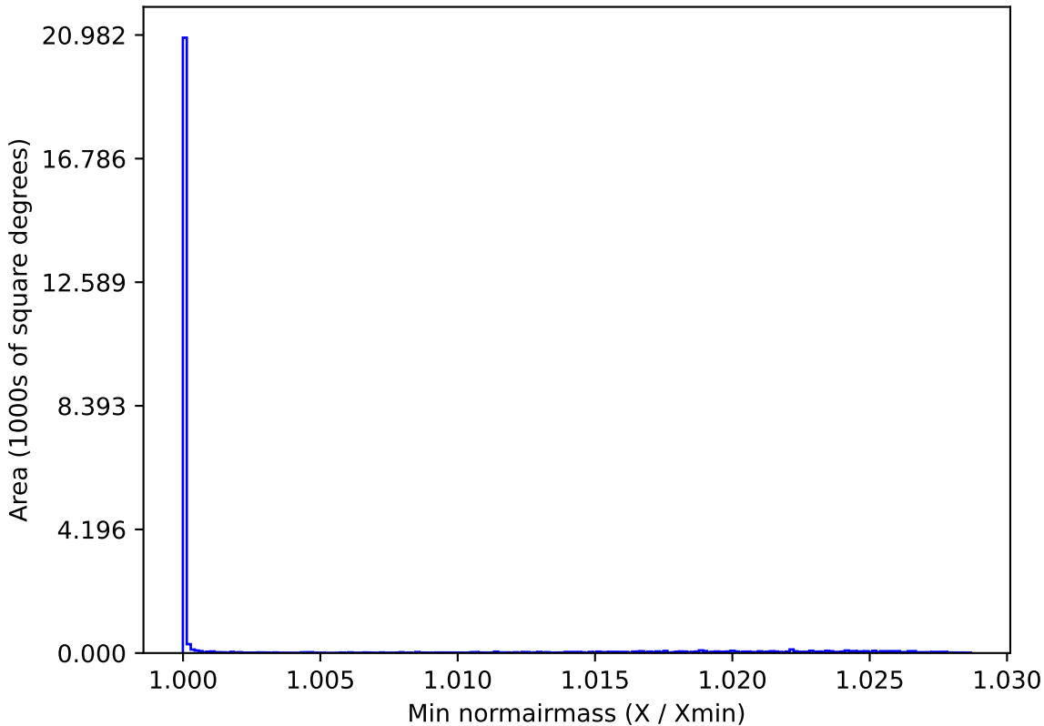
roll_pause_mjdp60_v3.4_10yrs All sky all bands: Min normairmass
