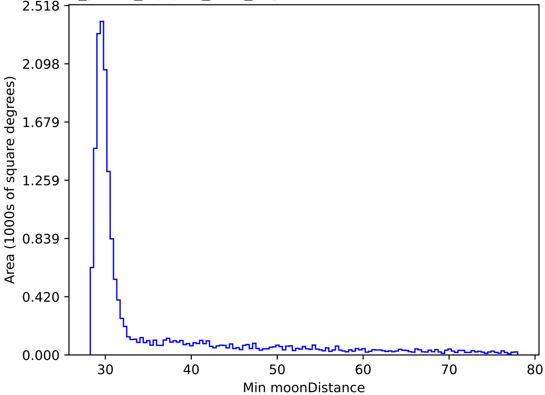
roll_pause_mjdp60_v3.4_10yrs WFD z band: Min moonDistance
