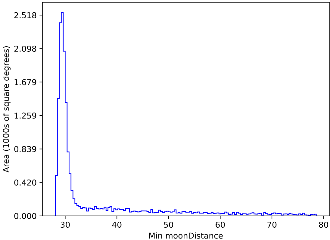
roll_pause_mjdp60_v3.4_10yrs WFD y band: Min moonDistance
