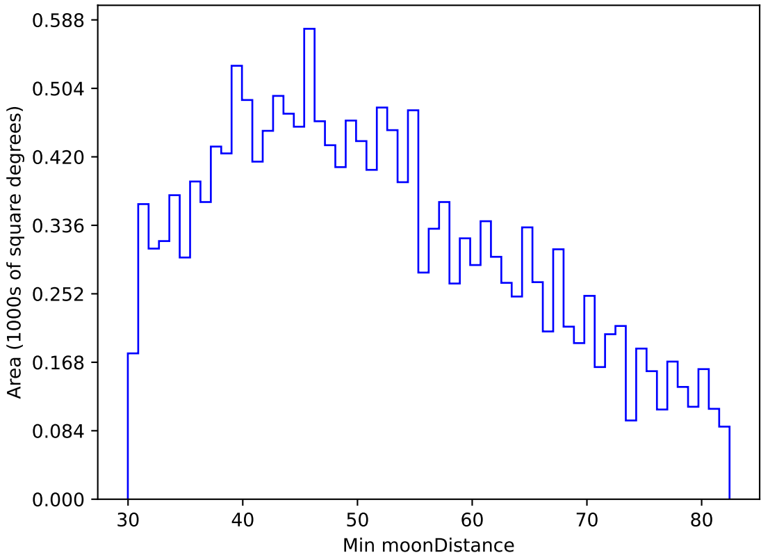
roll_pause_mjdp60_v3.4_10yrs WFD u band: Min moonDistance
