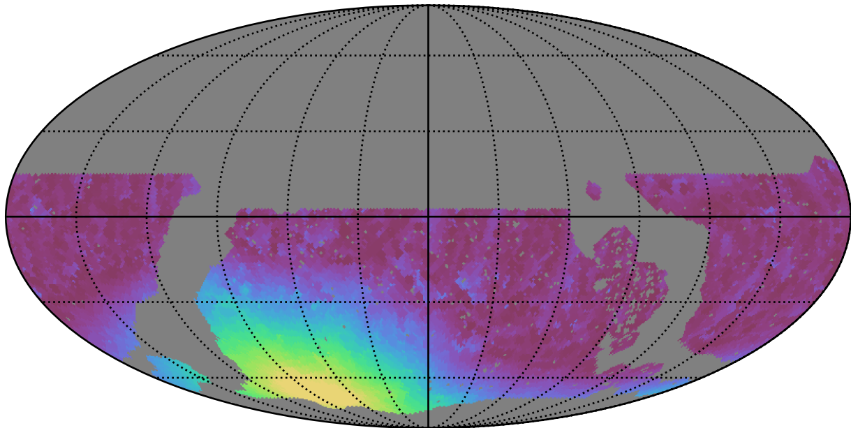
roll_pause_mjdp60_v3.4_10yrs WFD r band: Min moonDistance
