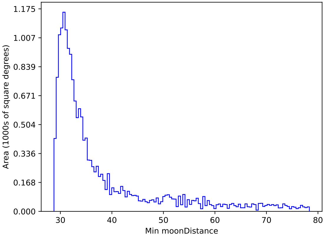
roll_pause_mjdp60_v3.4_10yrs WFD r band: Min moonDistance
