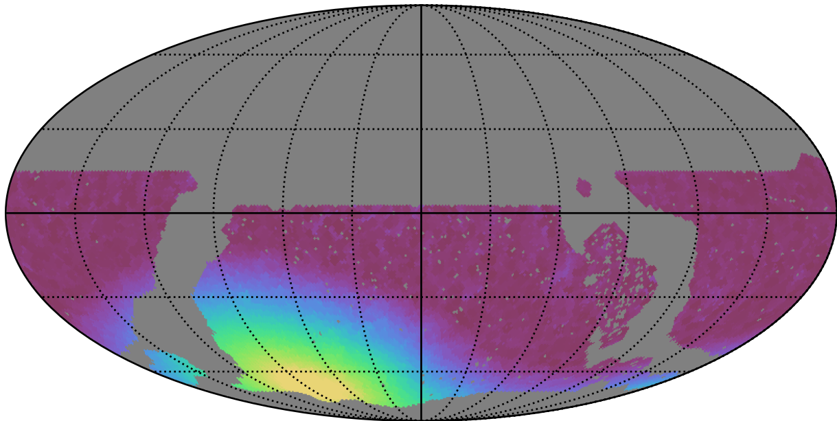
roll_pause_mjdp60_v3.4_10yrs WFD i band: Min moonDistance
