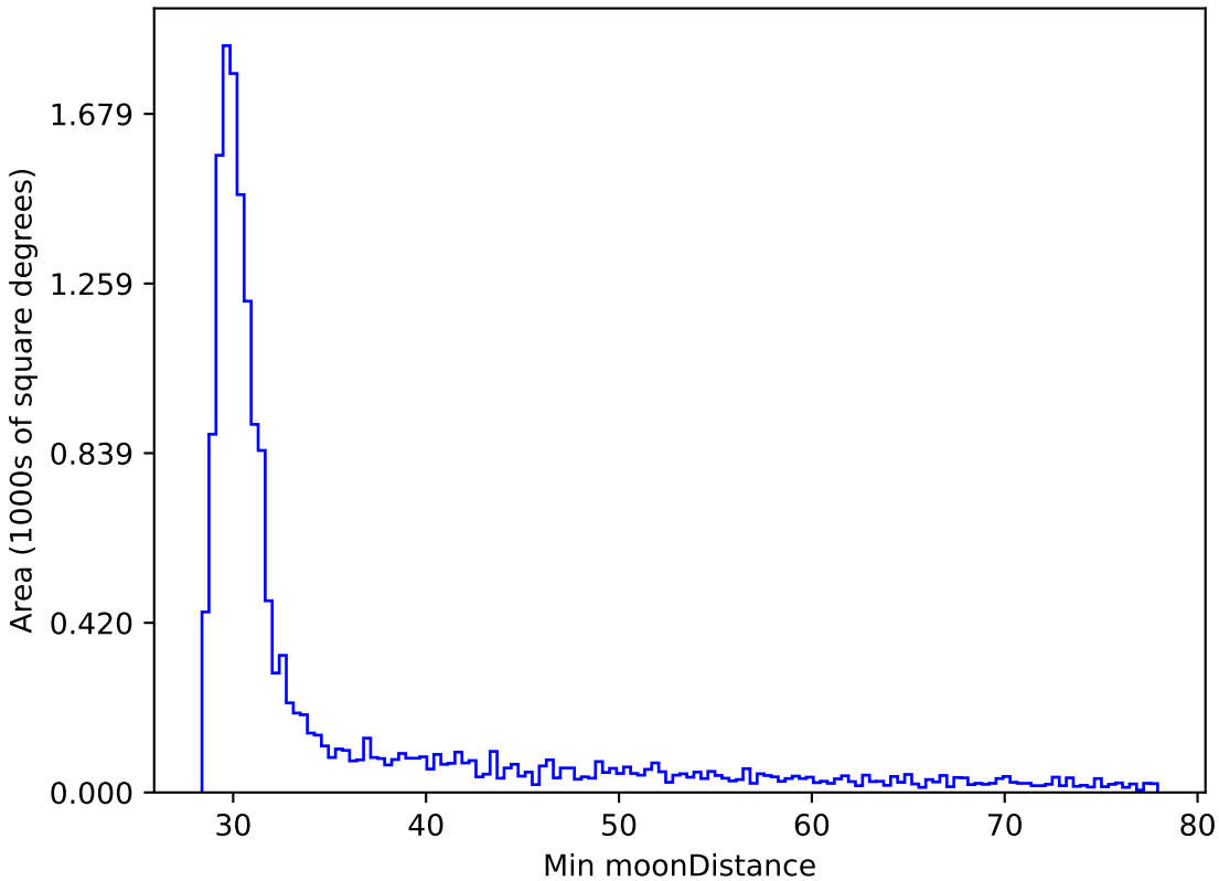
roll_pause_mjdp60_v3.4_10yrs WFD i band: Min moonDistance
