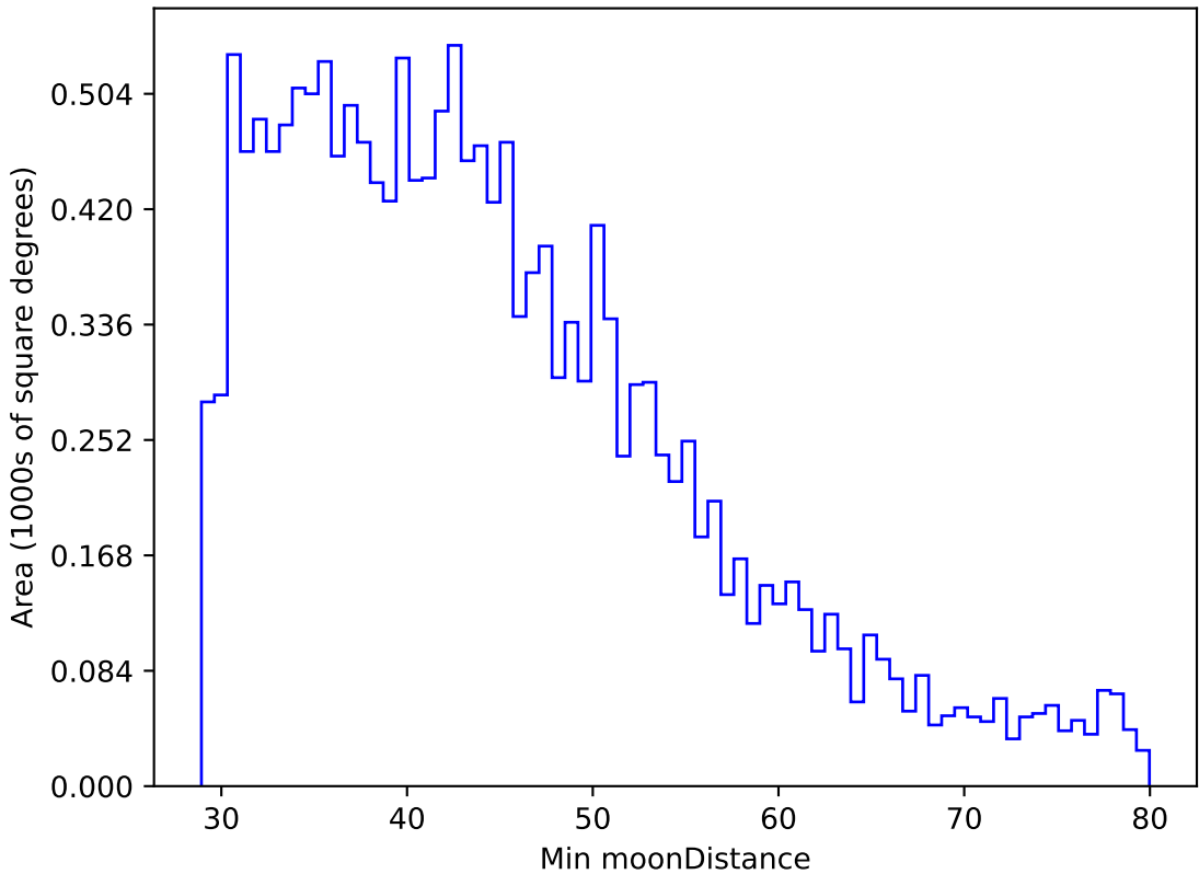
roll_pause_mjdp60_v3.4_10yrs WFD g band: Min moonDistance
