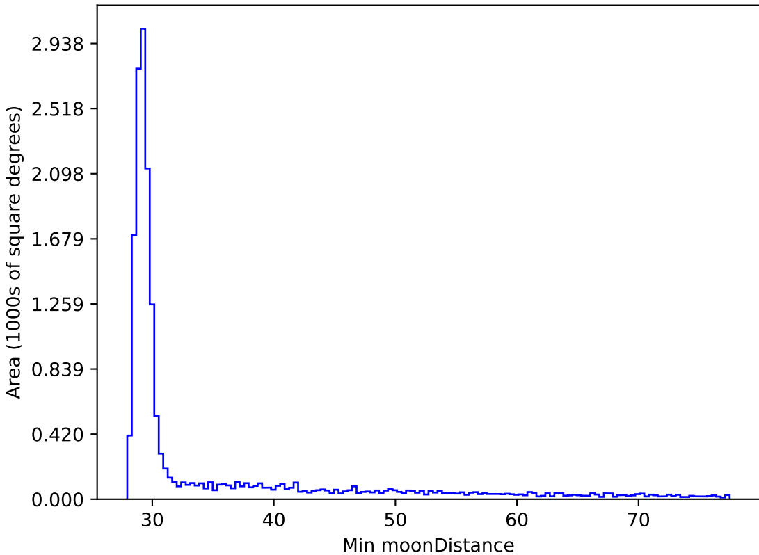
roll_pause_mjdp60_v3.4_10yrs WFD all bands: Min moonDistance
