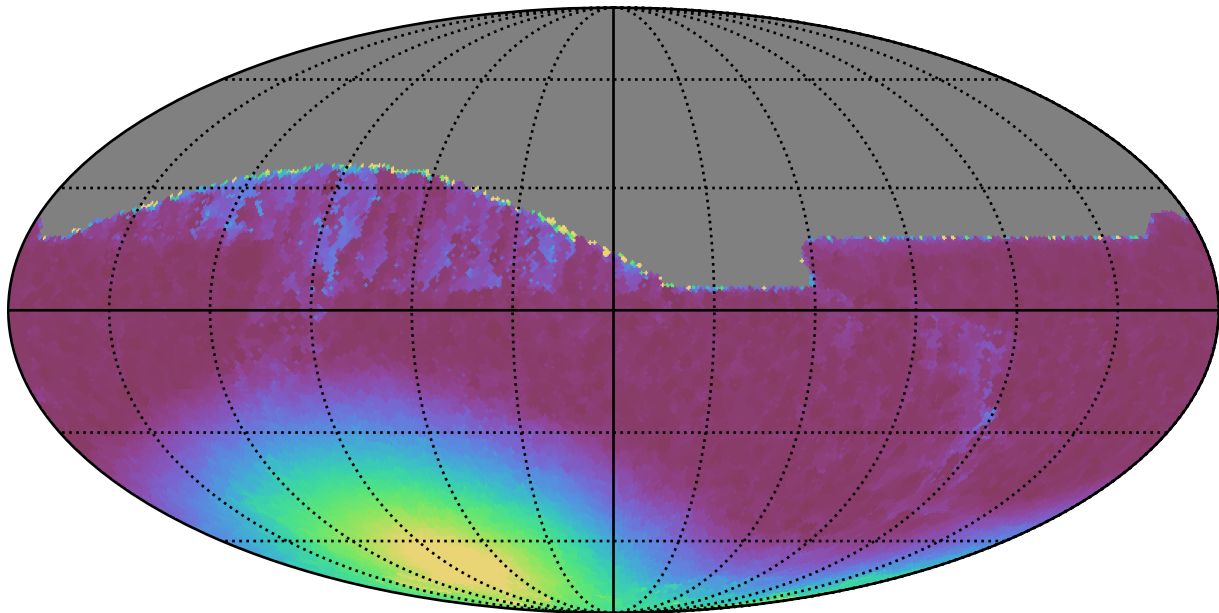
roll_pause_mjdp60_v3.4_10yrs All sky z band: Min moonDistance
