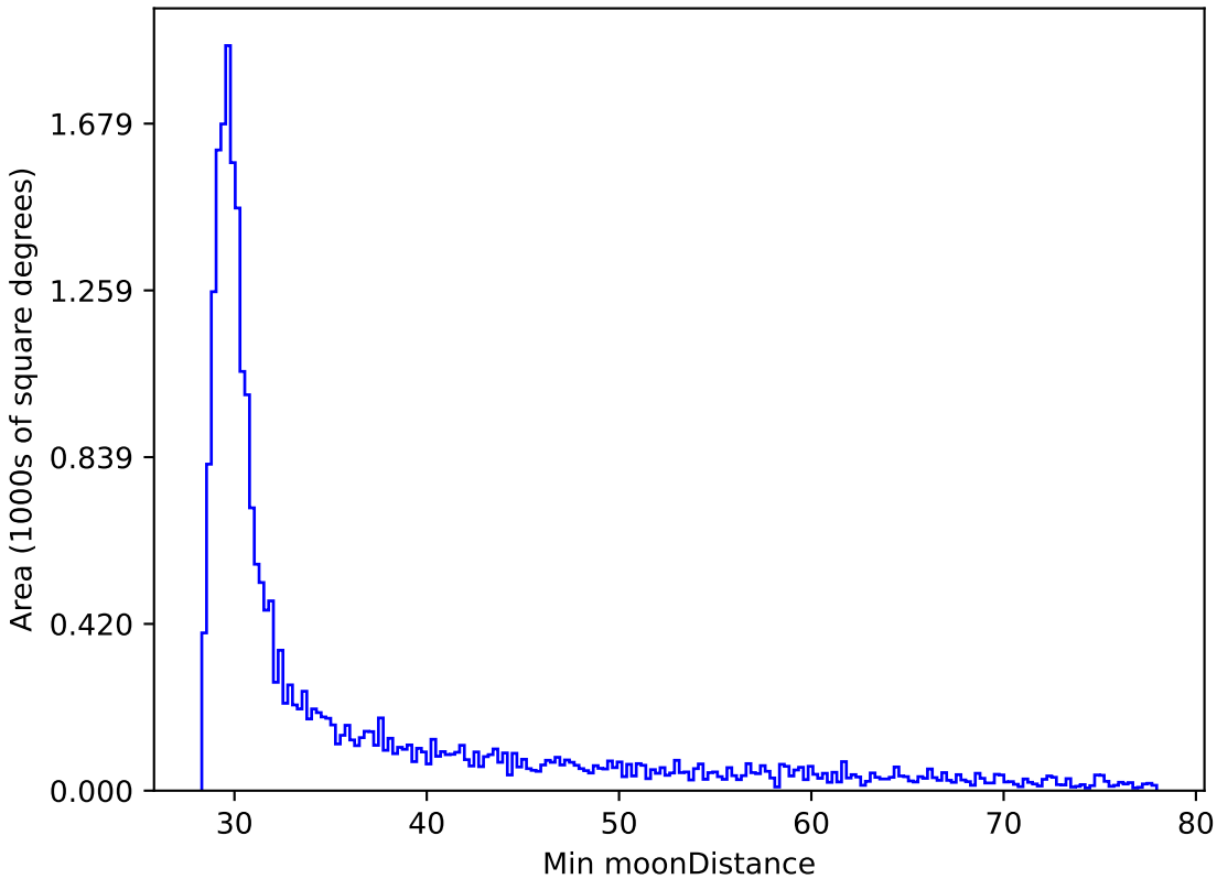
roll_pause_mjdp60_v3.4_10yrs All sky z band: Min moonDistance
