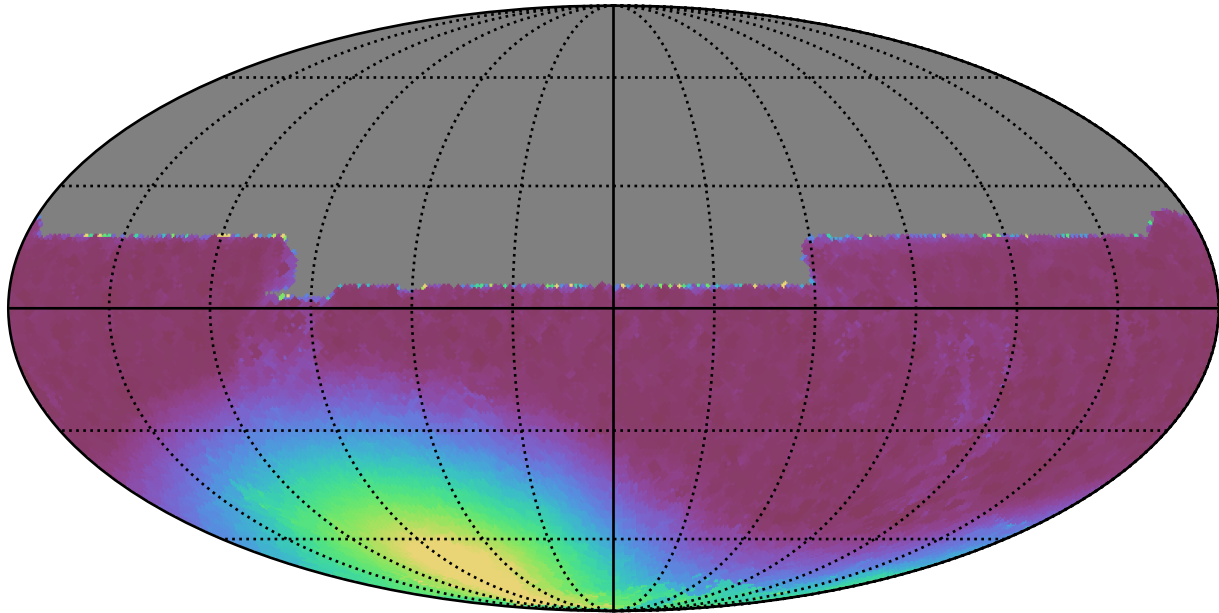
roll_pause_mjdp60_v3.4_10yrs All sky y band: Min moonDistance
