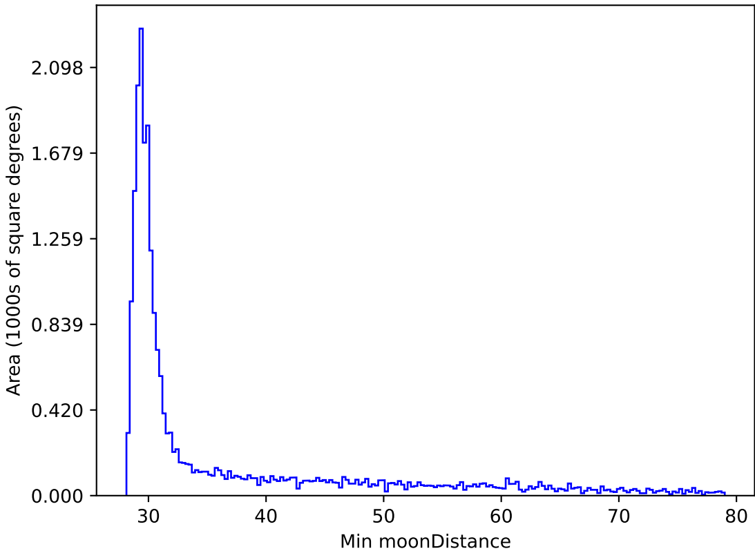
roll_pause_mjdp60_v3.4_10yrs All sky y band: Min moonDistance
