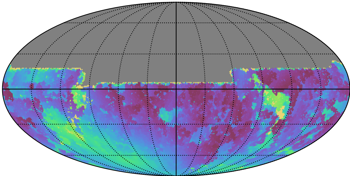
roll_pause_mjdp60_v3.4_10yrs All sky u band: Min moonDistance
