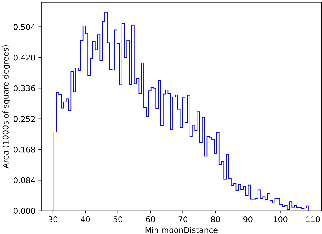
roll_pause_mjdp60_v3.4_10yrs All sky u band: Min moonDistance
