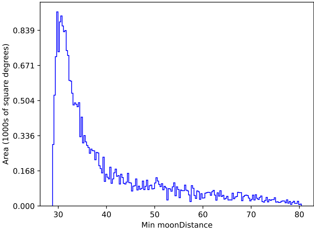
roll_pause_mjdp60_v3.4_10yrs All sky r band: Min moonDistance
