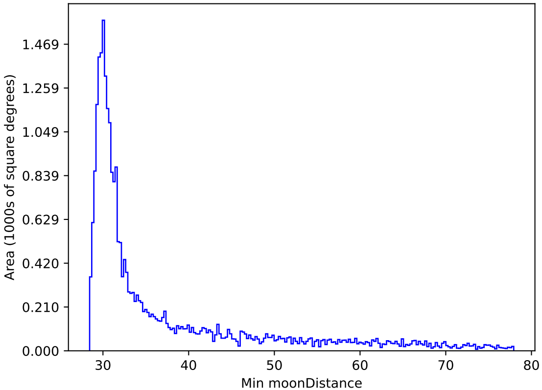
roll_pause_mjdp60_v3.4_10yrs All sky i band: Min moonDistance
