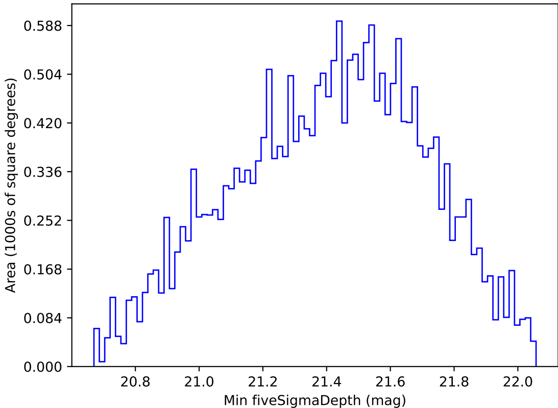
roll_pause_mjdp60_v3.4_10yrs Yr 1 y band: Min fiveSigmaDepth
