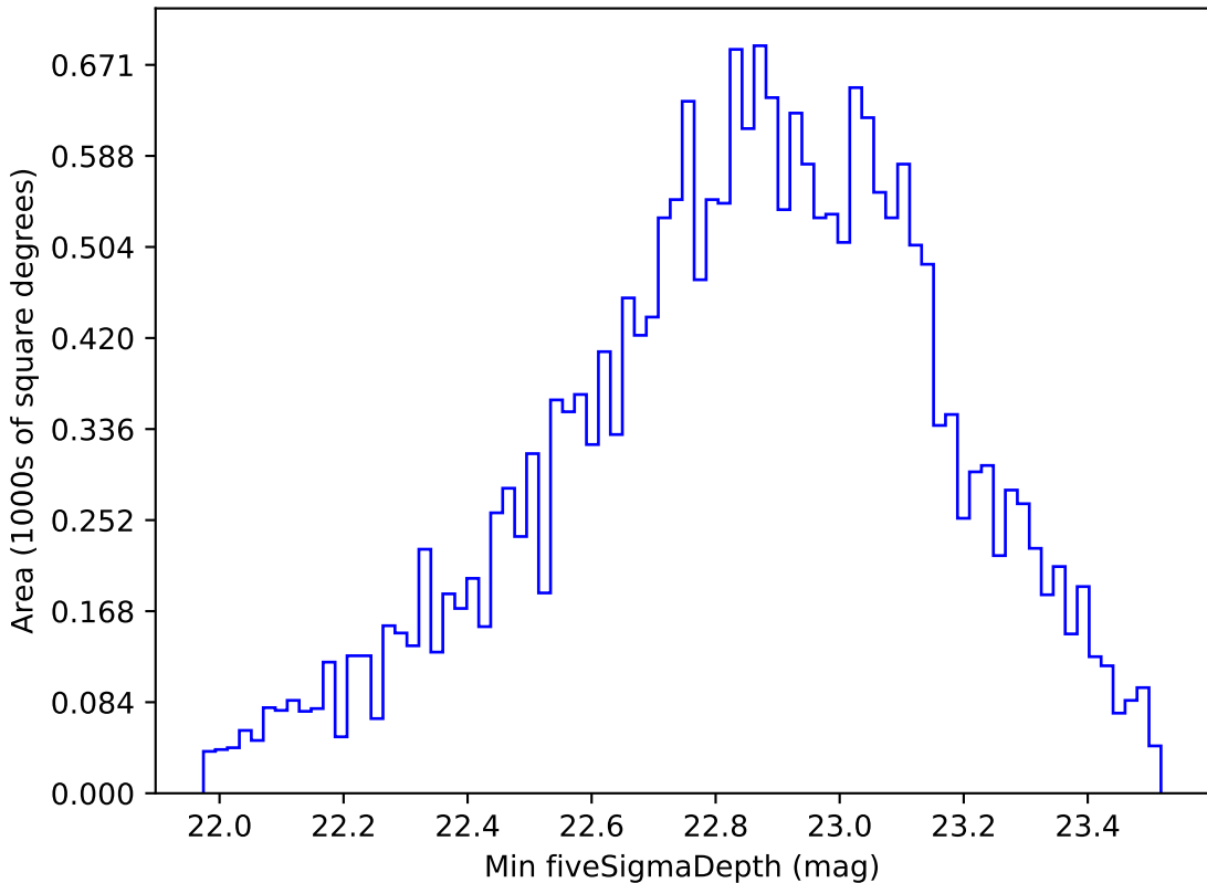
roll_pause_mjdp60_v3.4_10yrs Yr 1 u band: Min fiveSigmaDepth
