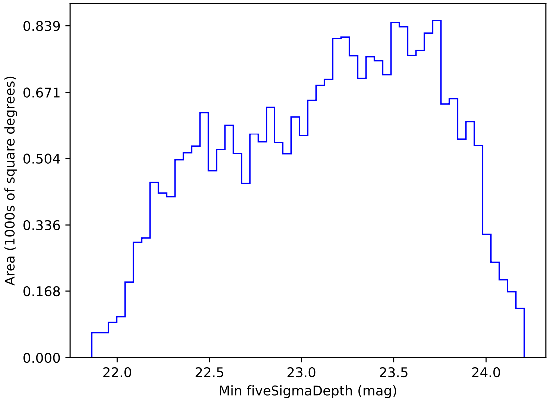
roll_pause_mjdp60_v3.4_10yrs Yr 1 r band: Min fiveSigmaDepth
