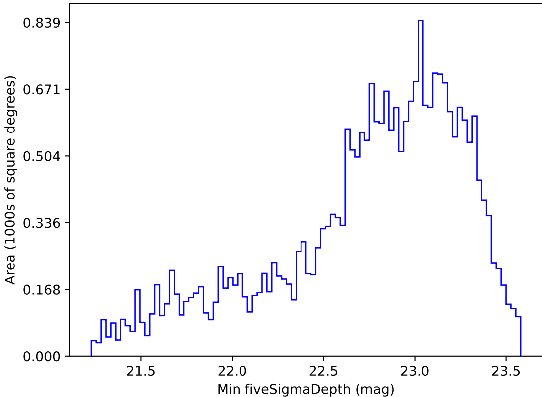
roll_pause_mjdp60_v3.4_10yrs Yr 1 i band: Min fiveSigmaDepth
