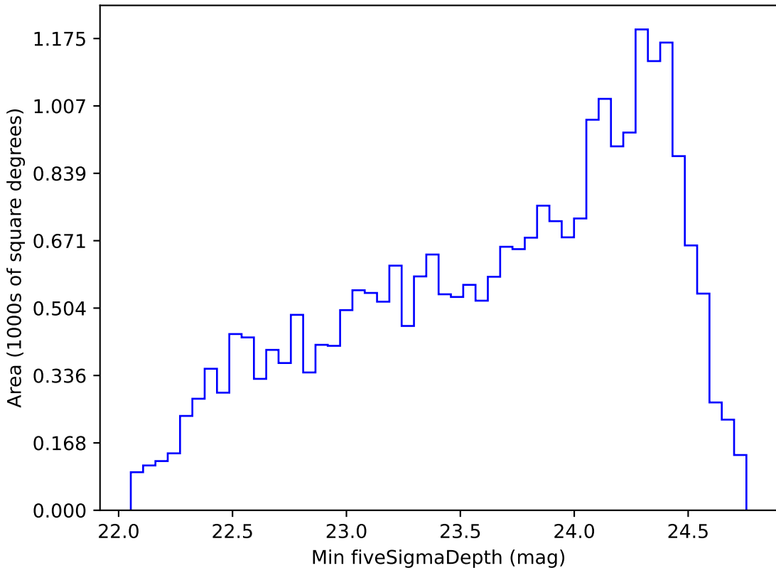
roll_pause_mjdp60_v3.4_10yrs Yr 1 g band: Min fiveSigmaDepth
