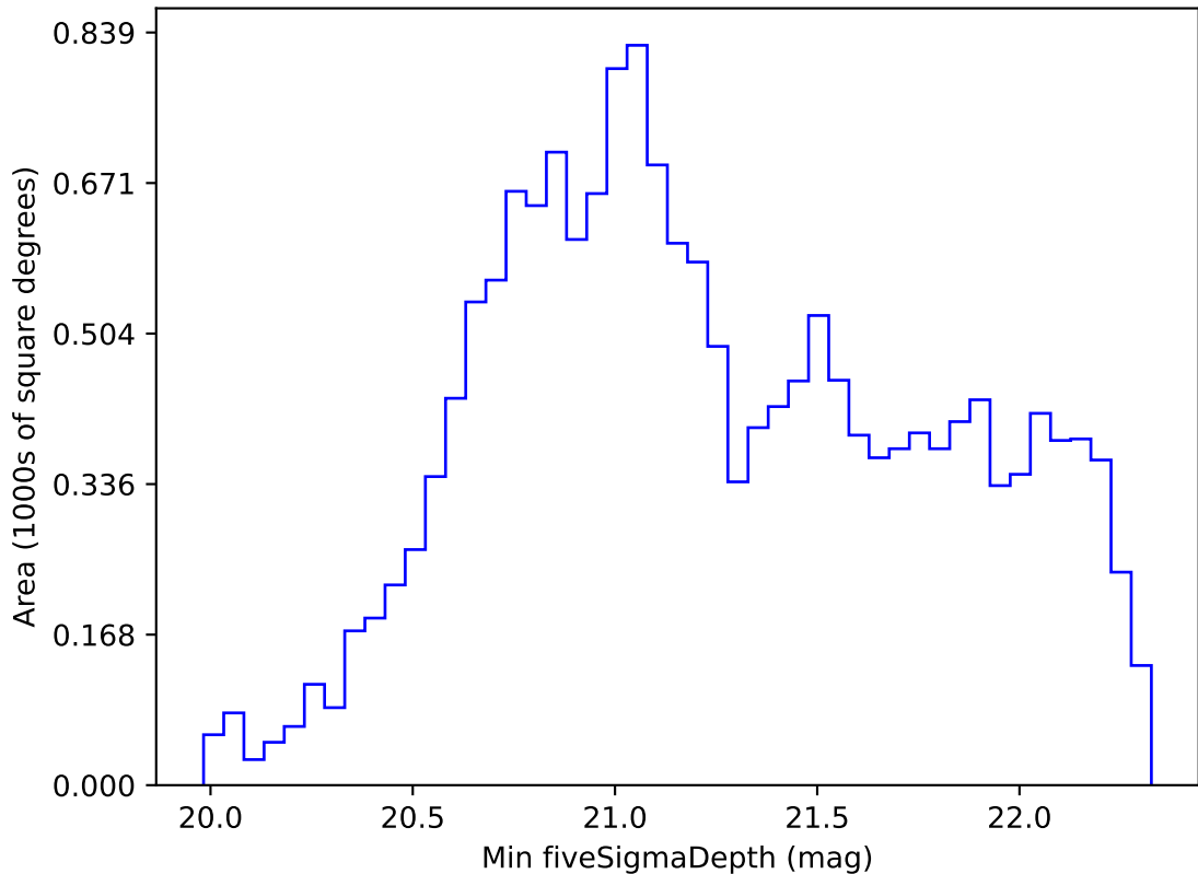
roll_pause_mjdp60_v3.4_10yrs WFD z band: Min fiveSigmaDepth
