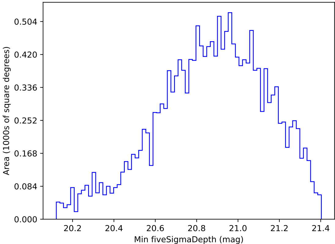
roll_pause_mjdp60_v3.4_10yrs WFD y band: Min fiveSigmaDepth
