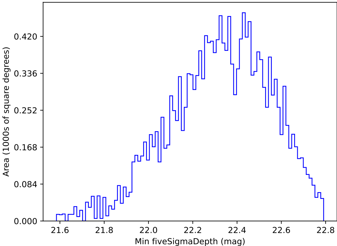
roll_pause_mjdp60_v3.4_10yrs WFD u band: Min fiveSigmaDepth
