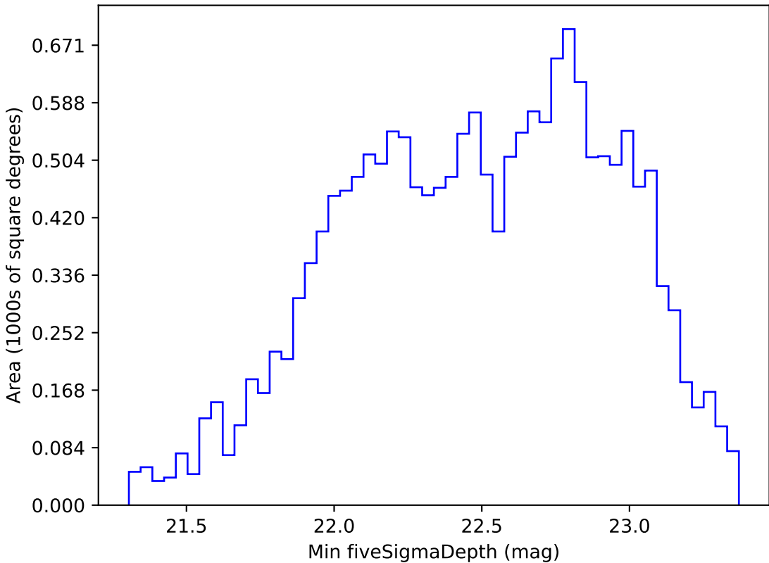
roll_pause_mjdp60_v3.4_10yrs WFD r band: Min fiveSigmaDepth
