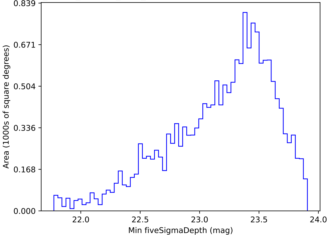
roll_pause_mjdp60_v3.4_10yrs WFD g band: Min fiveSigmaDepth
