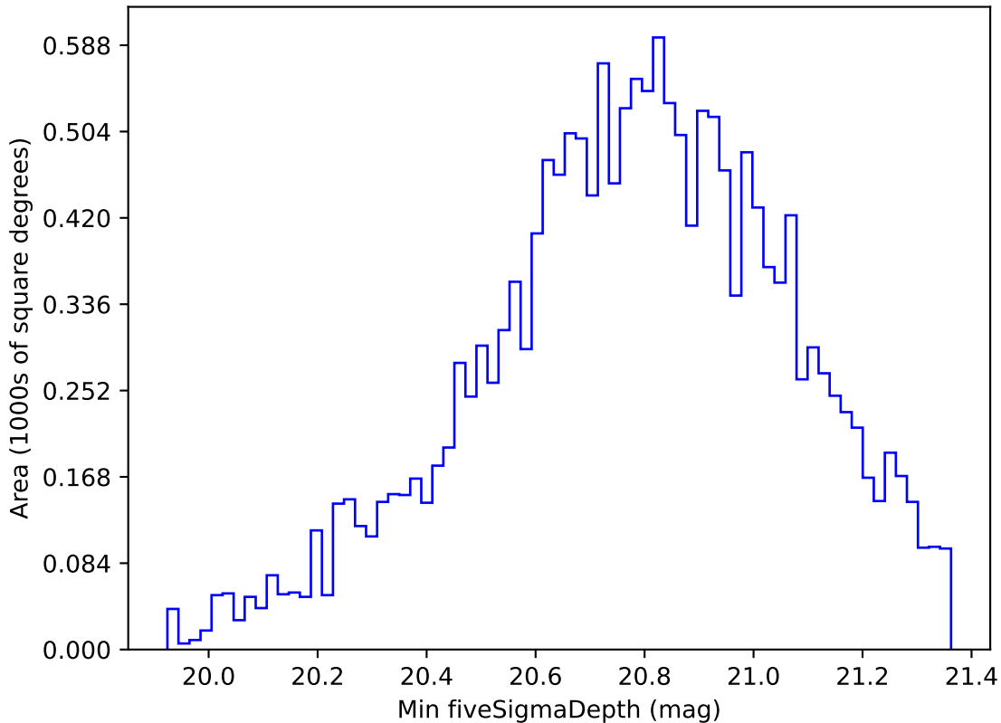
roll_pause_mjdp60_v3.4_10yrs WFD all bands: Min fiveSigmaDepth
