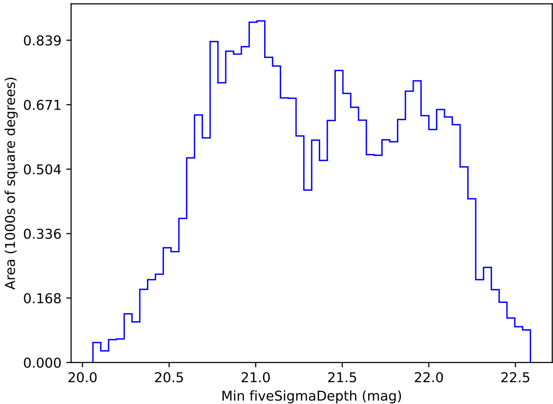
roll_pause_mjdp60_v3.4_10yrs All sky z band: Min fiveSigmaDepth
