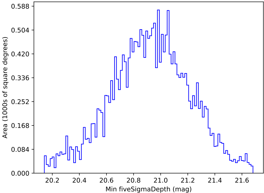
roll_pause_mjdp60_v3.4_10yrs All sky y band: Min fiveSigmaDepth
