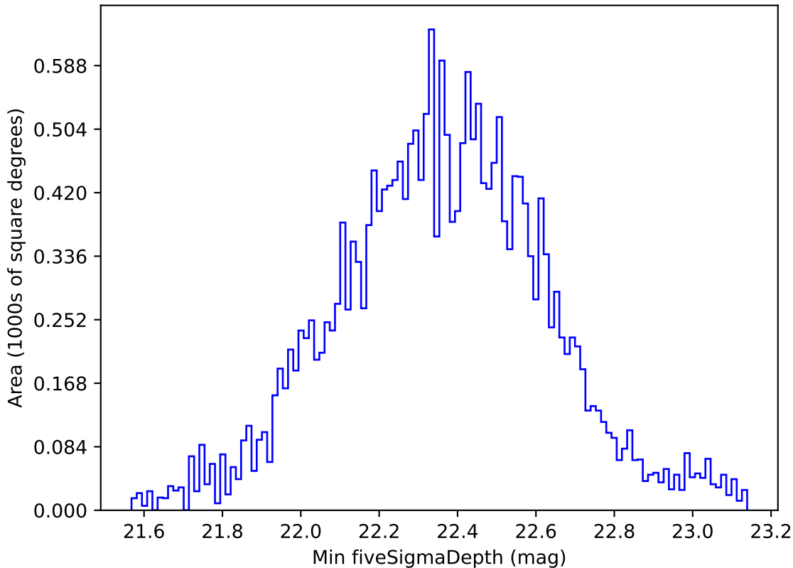
roll_pause_mjdp60_v3.4_10yrs All sky u band: Min fiveSigmaDepth
