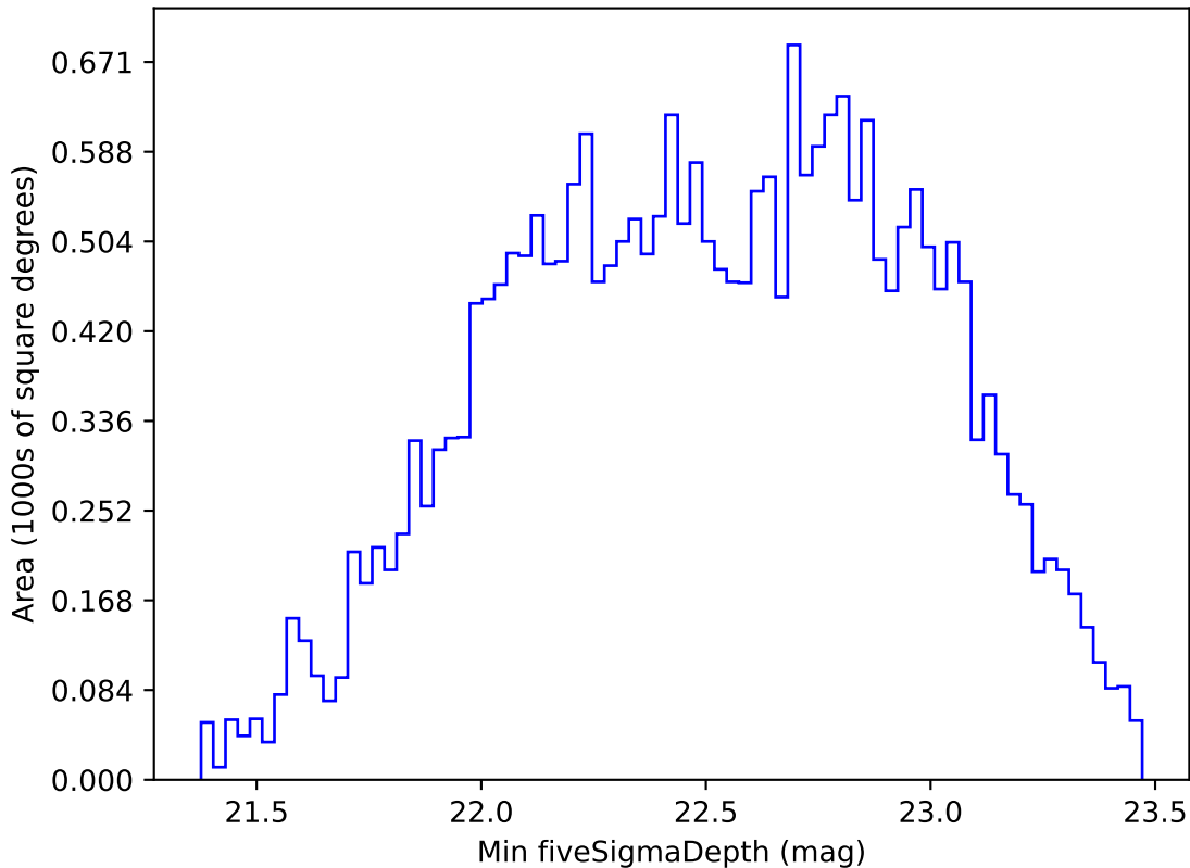
roll_pause_mjdp60_v3.4_10yrs All sky r band: Min fiveSigmaDepth
