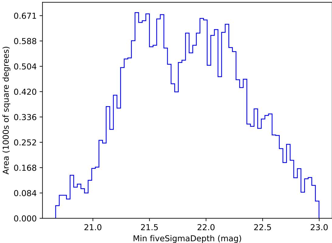
roll_pause_mjdp60_v3.4_10yrs All sky i band: Min fiveSigmaDepth
