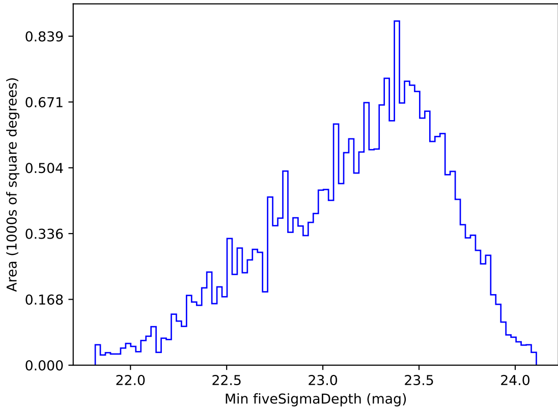
roll_pause_mjdp60_v3.4_10yrs All sky g band: Min fiveSigmaDepth
