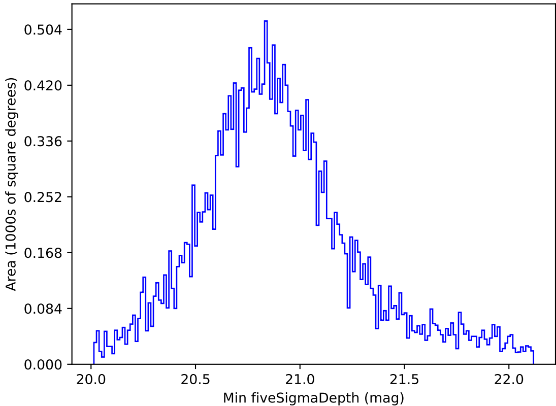
roll_pause_mjdp60_v3.4_10yrs All sky all bands: Min fiveSigmaDepth
