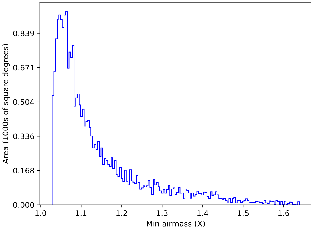
roll_pause_mjdp60_v3.4_10yrs Yr 1 u band: Min airmass
