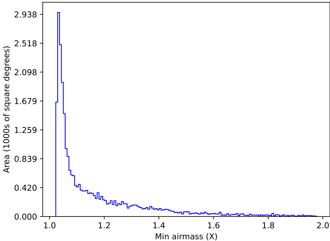
roll_pause_mjdp60_v3.4_10yrs Yr 1 r band: Min airmass
