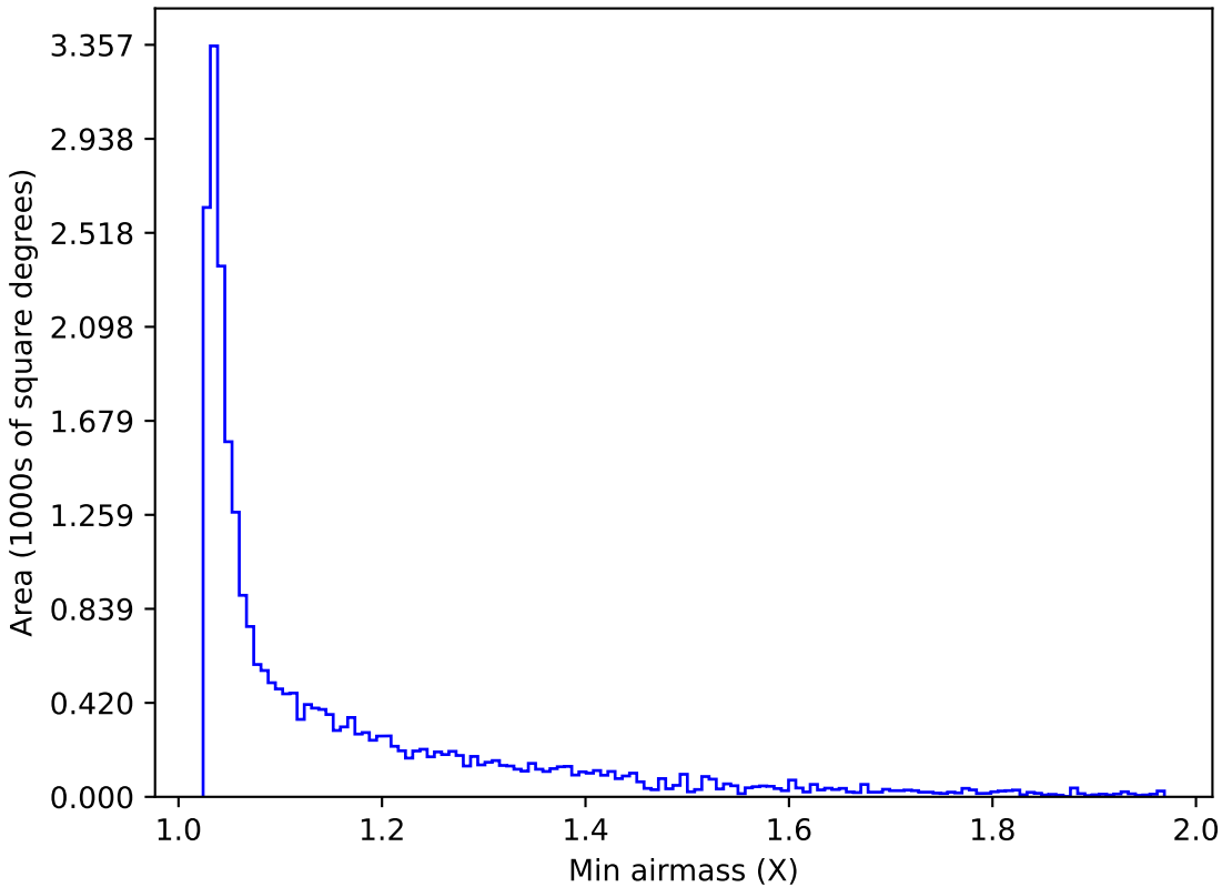
roll_pause_mjdp60_v3.4_10yrs Yr 1 i band: Min airmass
