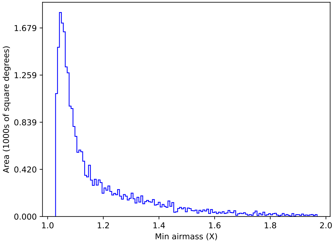
roll_pause_mjdp60_v3.4_10yrs Yr 1 g band: Min airmass
