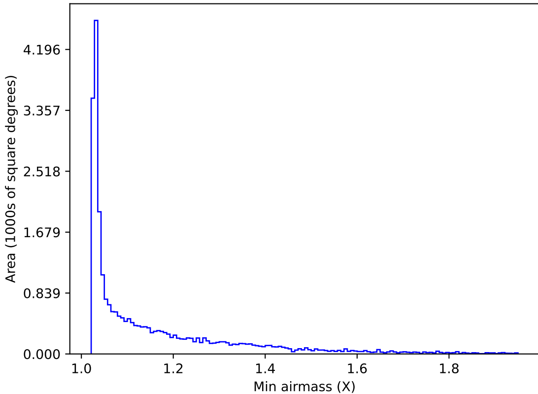
roll_pause_mjdp60_v3.4_10yrs Yr 1 all bands: Min airmass
