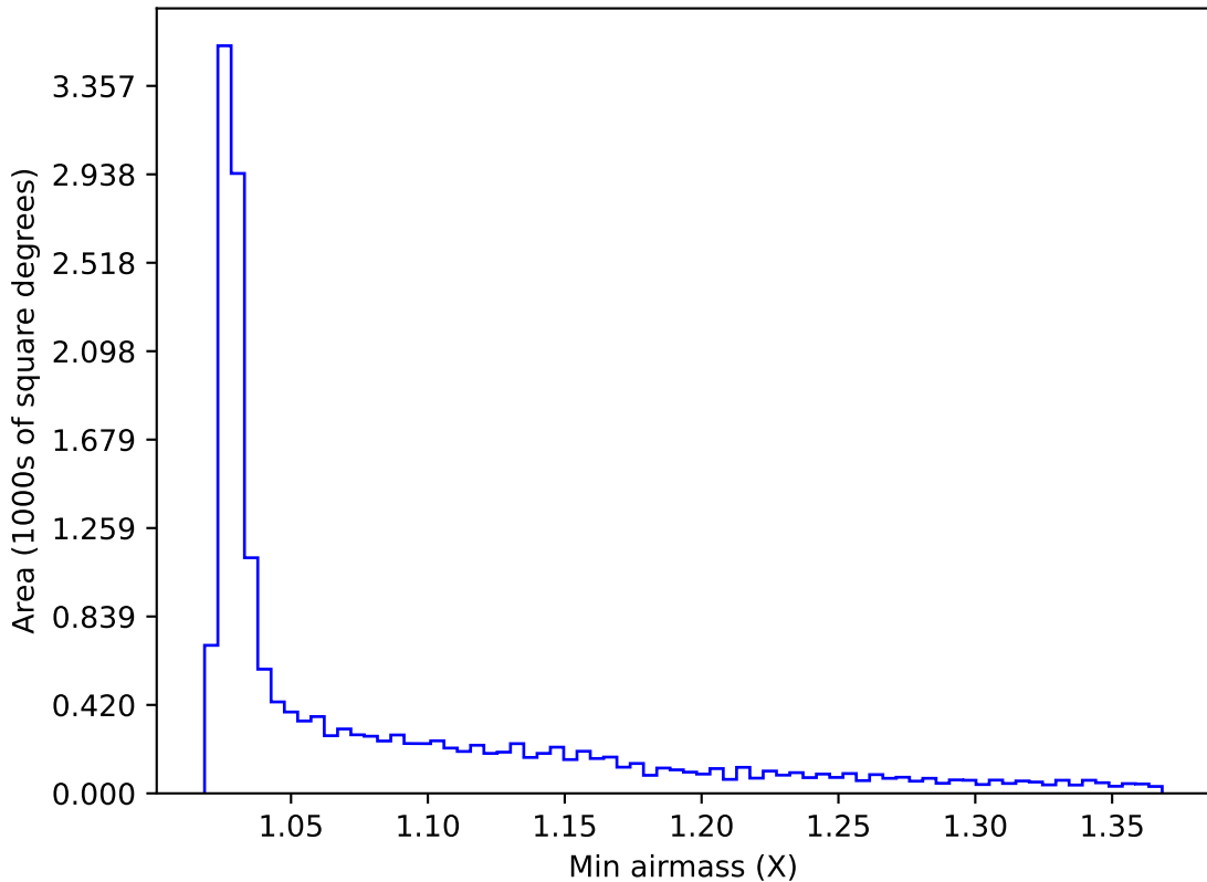
roll_pause_mjdp60_v3.4_10yrs WFD z band: Min airmass
