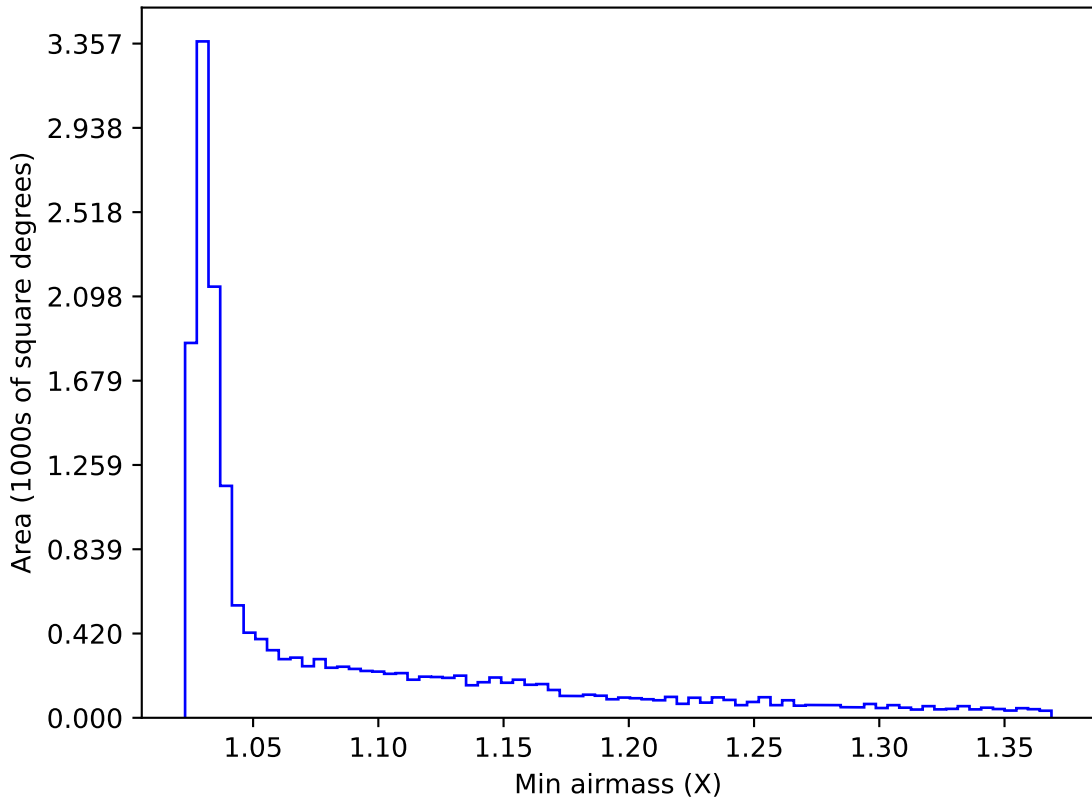
roll_pause_mjdp60_v3.4_10yrs WFD y band: Min airmass
