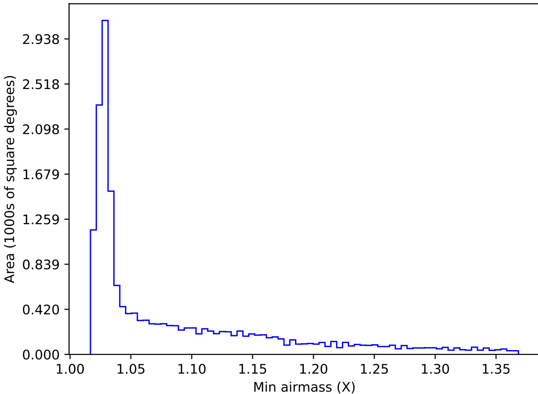
roll_pause_mjdp60_v3.4_10yrs WFD r band: Min airmass
