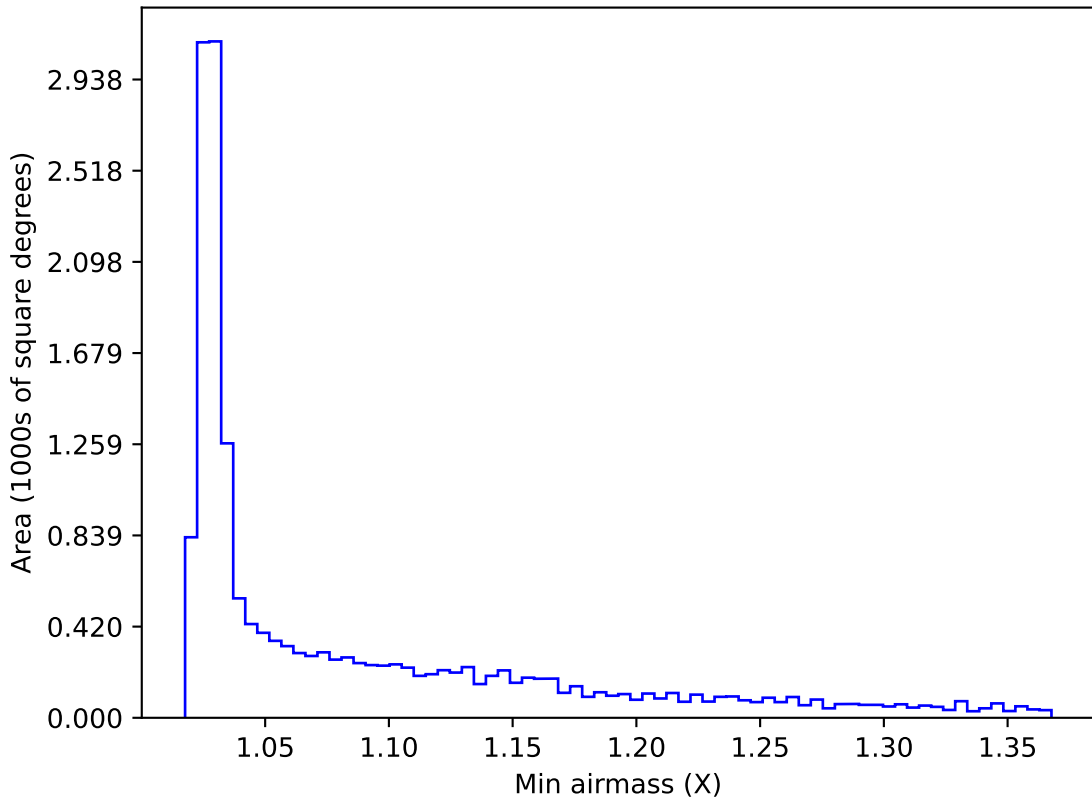
roll_pause_mjdp60_v3.4_10yrs WFD i band: Min airmass
